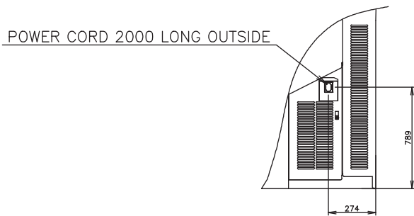
VIEW A(1/10)
